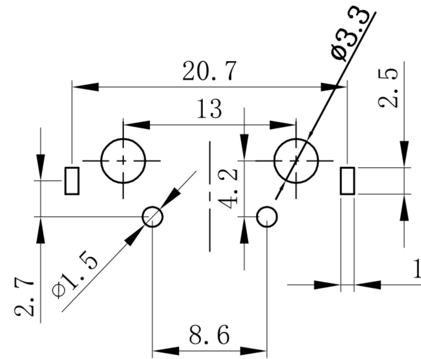
PCB LAYOUT
